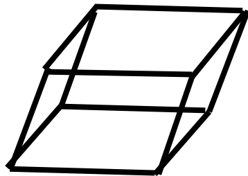
Rhombohedral
